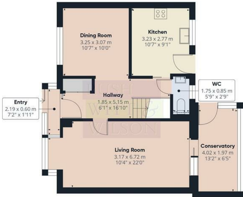
Floor 0 Building 1
